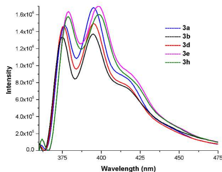
Figure 4: Emission spectra (excited at 350 nm, 25 °C, slit = 1/1) of compounds 3a-b , 3d-e , 3h in THF
