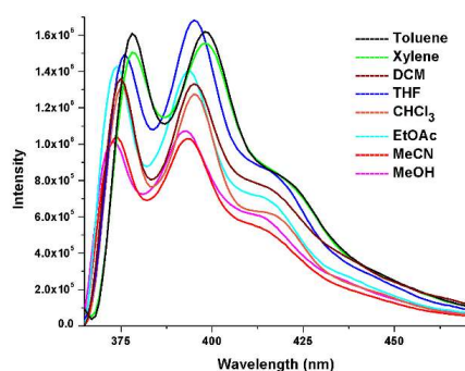
Figure 3: Solvatochromic effects on emission spectra of compound 3a (excited at 350 nm, 25°C, slit = 1/1).
