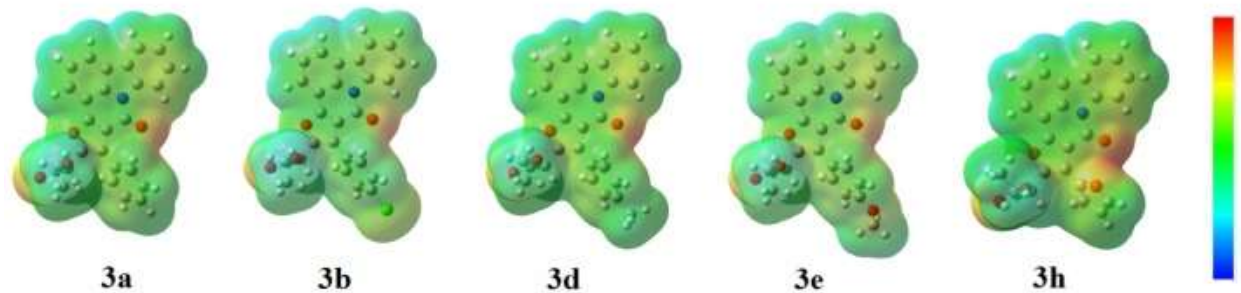
Figure 7. Molecular electrostatic potential (MEP) diagrams of all the compounds.
