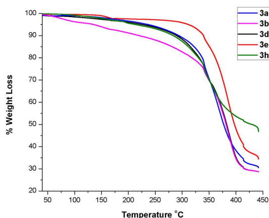
Figure 8. TGA spectra of compounds 3a-b , 3d-e and 3h .
