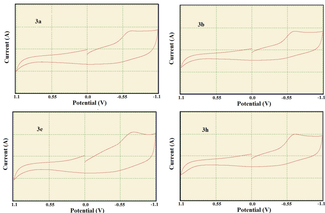
Figure 9. CV curves of 3a , 3b , 3e and 3h in DMF at pH 6.5, C = 1 \times 10^{-5} M.
