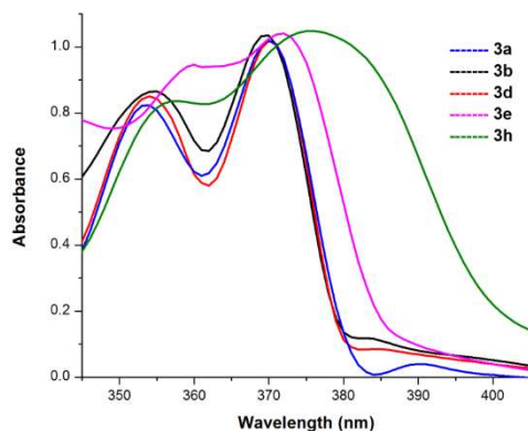
Figure 2. Normalized absorption spectra of compounds 3a-b , 3d-e , 3h in THF( 1 \times 10^{-5} M, 25°C).
