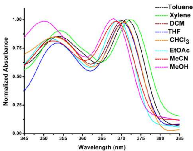
Figure 1. Solvatochromic effects on absorption spectra of compound 3a ( 1 \times 10^{-5} M, 25 °C).
